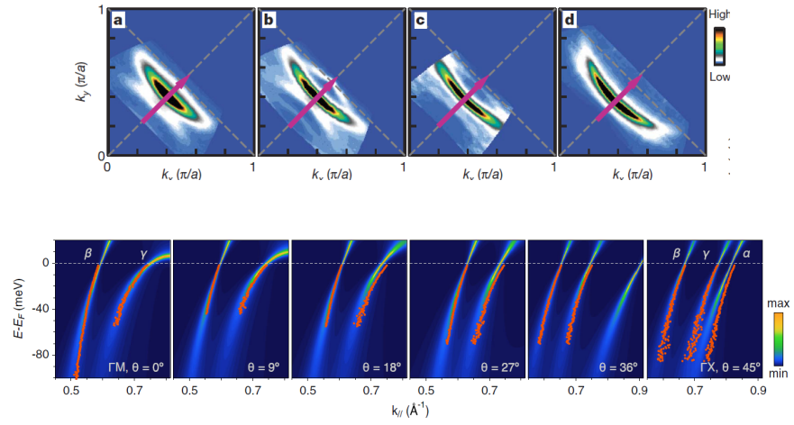
Figure 31-3 Comparison between theory and experiment for strontium ruthenate. The theory is from electronic structure including spin-orbit interactions and supplemented with the effect of interactions using Dynamical Mean-Field theory. From Phys. Rev. X, 2 , 021048 (2019).
