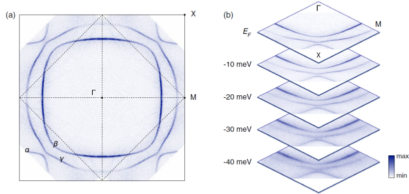
Figure 31-2 Momentum distribution curves. a) at the Fermi level, and b) at various energies below the Fermi surface. From Phys. Rev. X, 2 , 021048 (2019).
