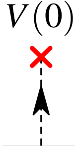
Figure 18-5 First-order irreducible self-energy.
