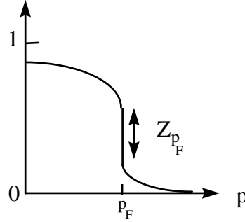
Figure 31-6 Qualitative sketch of the zero-temperature momentum distribution in an interacting system.
