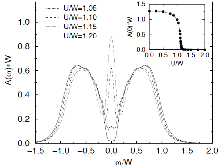
Figure 60-3 decrease for U 1:1 W; from Ref. [78] in Vollhardt in Mancini.
