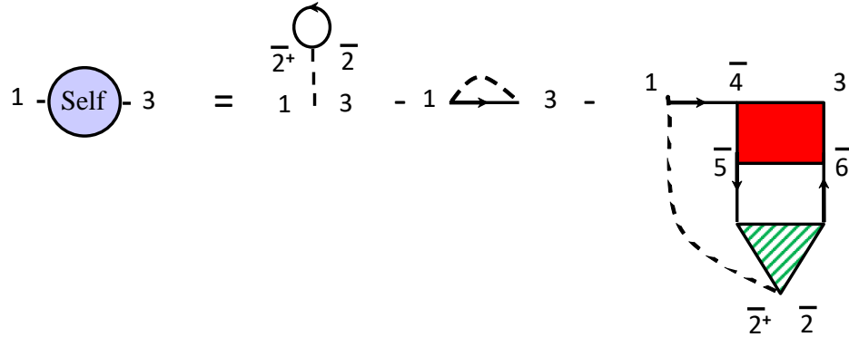
Figure 36-2 Diagrams for the self-energy. The dashed line represent the interaction. The first two terms are, respectively, the Hartree and the Fock contributions. The textured square appearing in the previous figure for the four-point function has been squeezed to a triangle to illustrate the fact that two of the indices (coordinates) are identical.
