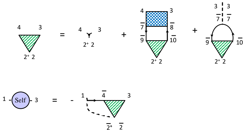
Figure 51-2 \delta\mathcal{G}/\delta\phi has been separated in two parts: the last term of the top line that comes from \delta\Sigma/\delta\mathcal{G} of the Hartree term in \Sigma and the blue box that represents the rest. That blue box appears both on the top and the bottom line. The top line is the same figure as the preceding one, but with the two external legs amputated. Comparing with the equation for the self-energy in the previous figure, we see that the self-energy can now be written entirely in terms of the green triangle, also known as fully reducible vertex.
