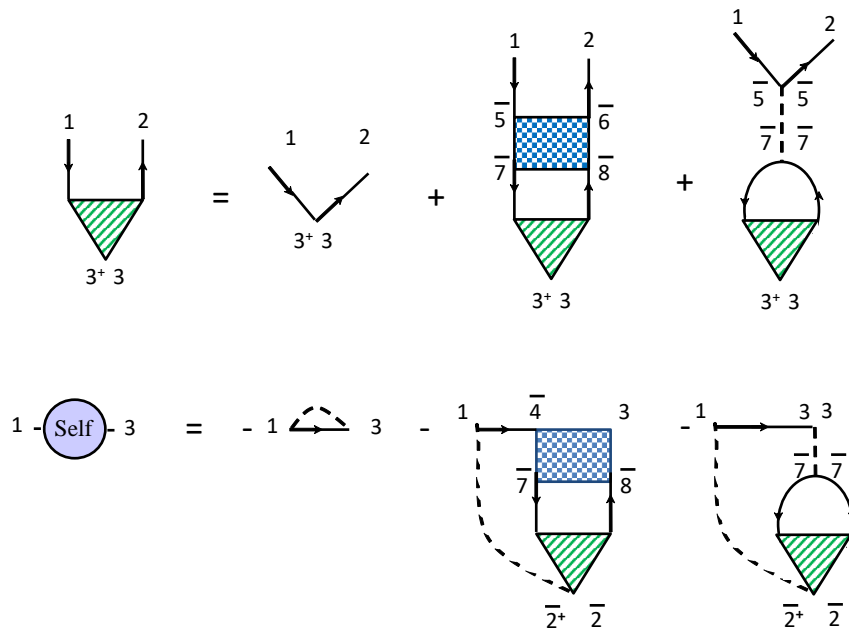
Figure 51-1 Rewriting our two equations for \delta\mathcal{G}/\delta\phi and for \Sigma in such a way that the Hartree term has been absorbed in a redefinition of the chemical potential and the irreducible vertex that was the red box entering the equation for \delta\mathcal{G}/\delta\phi has been separated in two parts: the last term of the top line that comes from \delta\Sigma/\delta\mathcal{G} of the Hartree term in \Sigma and the blue box that represents the derivative of the rest of \Sigma that appears on the bottom line. The green triangle, as before, is the fully reducible vertex.
