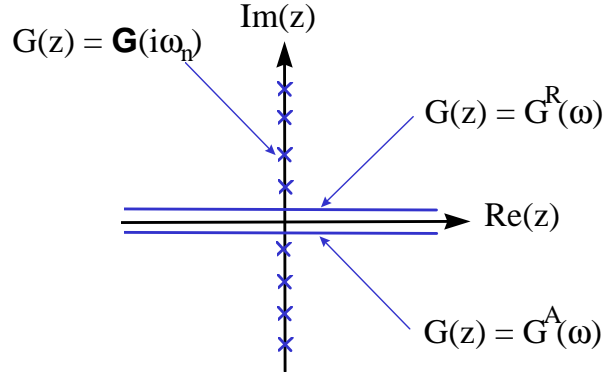
Figure 29-3 Analytical structure of G(z) in the complex frequency plane. G(z) reduces to either G^R(\omega) , G^A(\omega) or \mathcal{G}(i\omega_n) depending on the value of the complex frequency z . There is a branch cut along the real axis.
