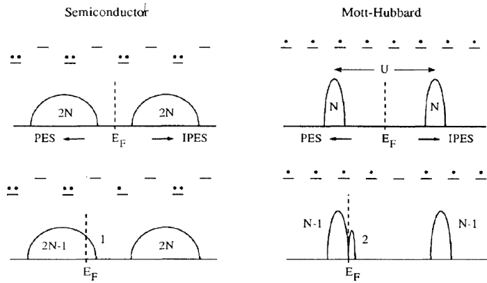
Figure 60-3 decrease for U 1:1 W; from Ref. [78] in Vollhardt in Mancini.
