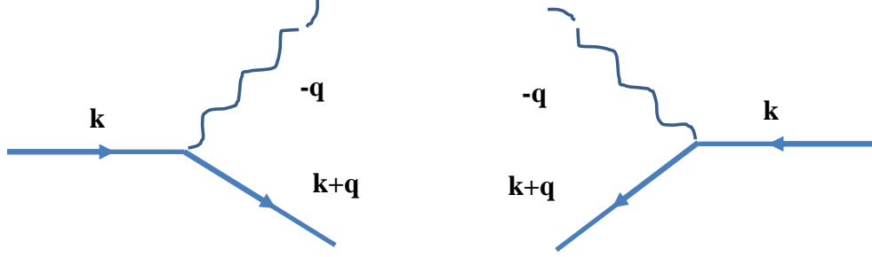
Figure 45-3 Schematic representation of the processes contained in the imaginary part of the self-energy. On the left, an electron with momentum and frequency \mathbf{k}, \omega decays into another a quasiparticle \mathbf{k} + \mathbf{q}, \zeta_{\mathbf{k}+\mathbf{q}} plus a particle-hole excitation -\mathbf{q}, \omega - \zeta_{\mathbf{k}+\mathbf{q}} that can be a plasmon, depending on the conditions on wave-vector and frequency. On the right, the analogous process for a hole.
