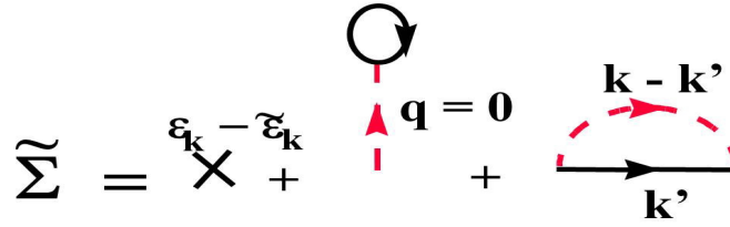
Figure 42-3 Effective medium point of view for the Hartree-Fock approximation. In this figure, the propagators are evaluated with the effective medium \tilde{H}_0 . The Hartree term is known as the tadpole diagram and the Fock term as the sunrise diagram.
