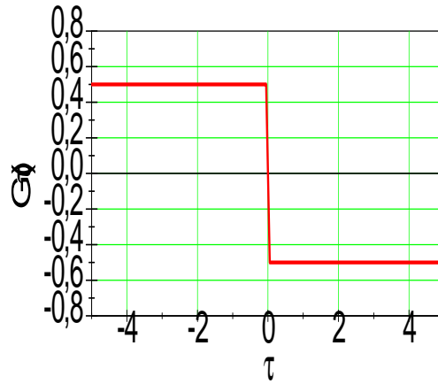
Figure 29-5 \mathcal{G}_0(\mathbf{p}, \tau) for a value of momentum at the Fermi surface.
