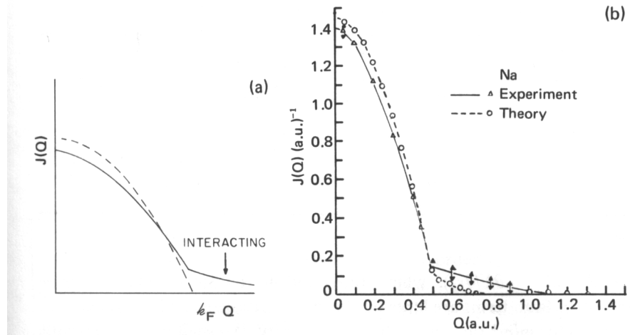
Figure 45-6 a) Dashed line shows the momentum distribution in Compton scattering for the non-interacting case while the solid line is for an interacting system. b) Experimental results in metallic sodium compared with theory, r_s = 3.96 . Eisenberger et al. Phys. Rev. B 6 , 3671 (1972).
