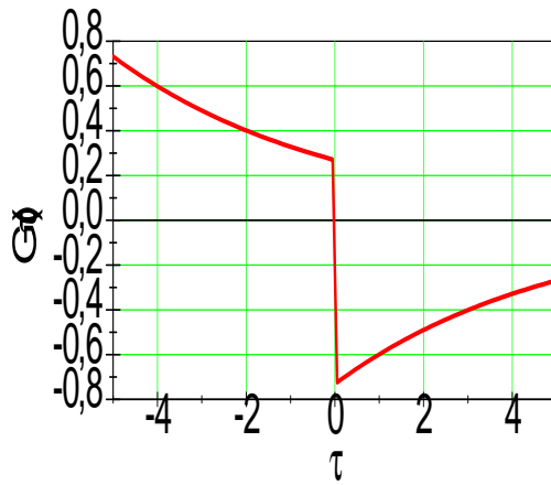
Figure 29-4 \mathcal{G}_0(\mathbf{p}, \tau) for a value of momentum above the Fermi surface.
