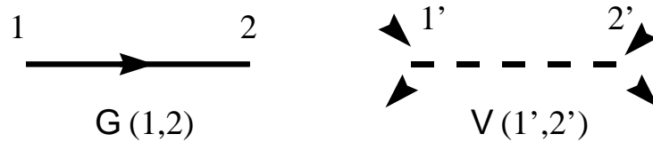
Figure 38-1 Basic building blocks of Feynman diagrams for the electron gas.
