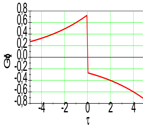
Figure 29-6 \mathcal{G}_0(\mathbf{p}, \tau) for a value of momentum below the Fermi surface.
